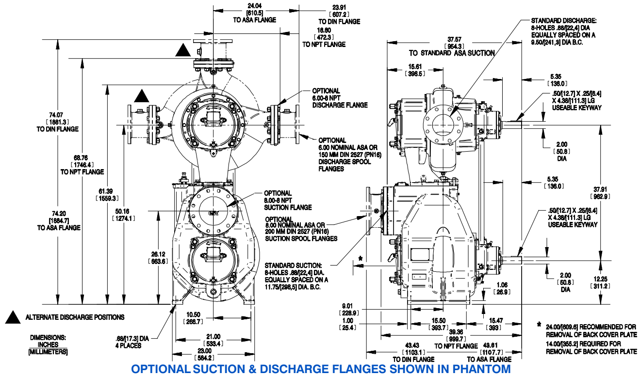
OPTIONAL SUCTION & DISCHARGE FLANGES SHOWN IN PHANTOM
