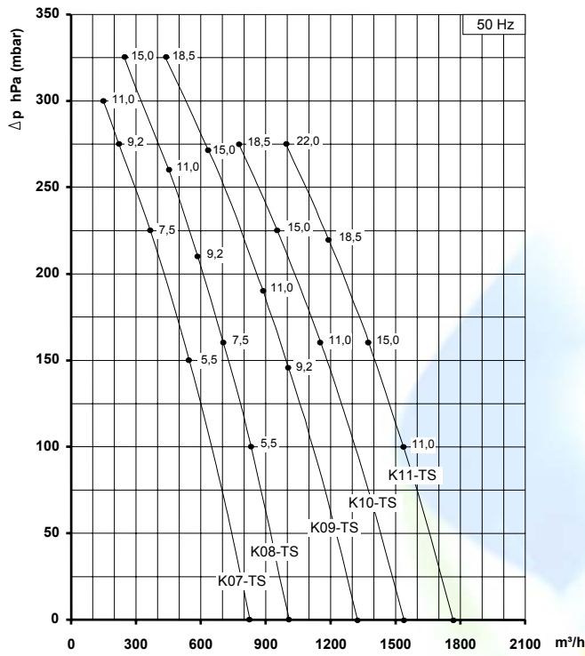
CAPACITY
