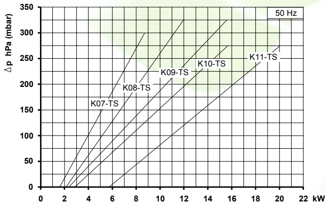
ABSORBED POWER
